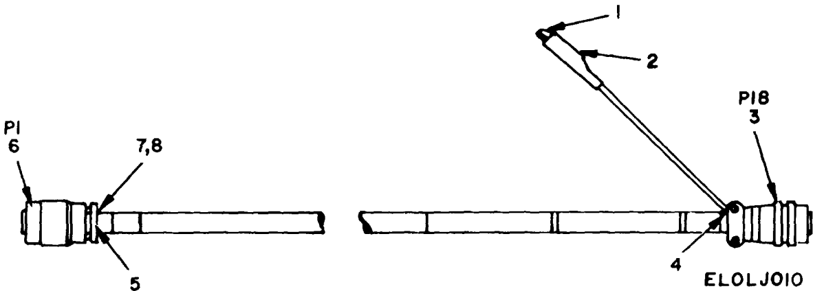
Figure 10. Cable Assembly CX-8784/ASM-125, W9.
