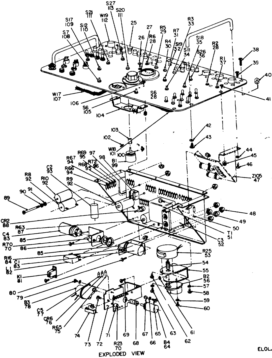
Figure 18. Chassis Assembly (Sheet 2 of 3).
