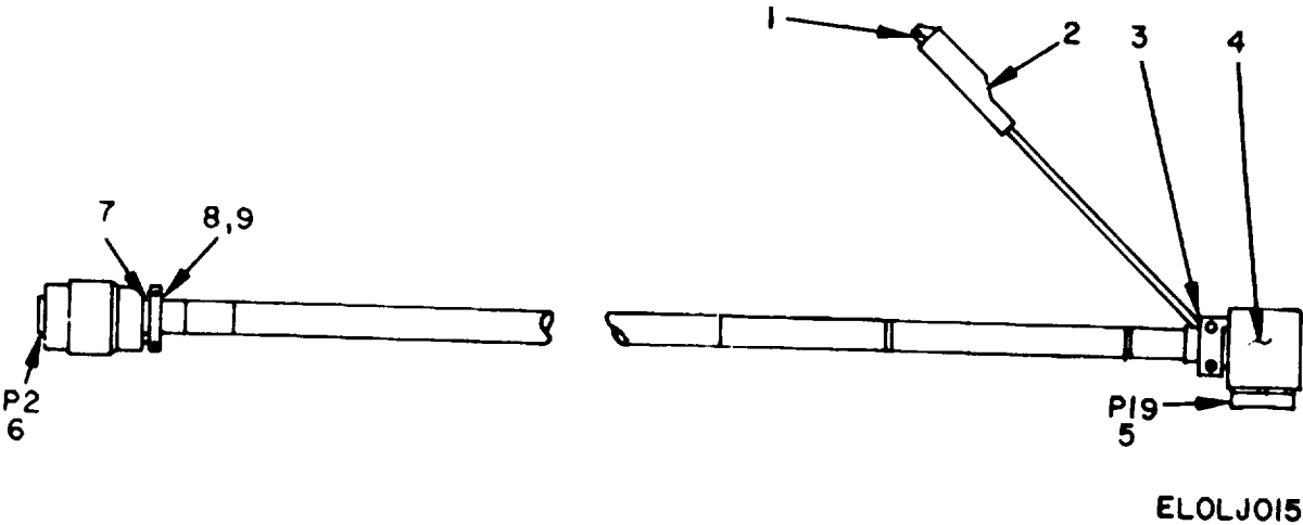
Figure 15. Cable Assembly CX-8785/ASM-125, W14.
