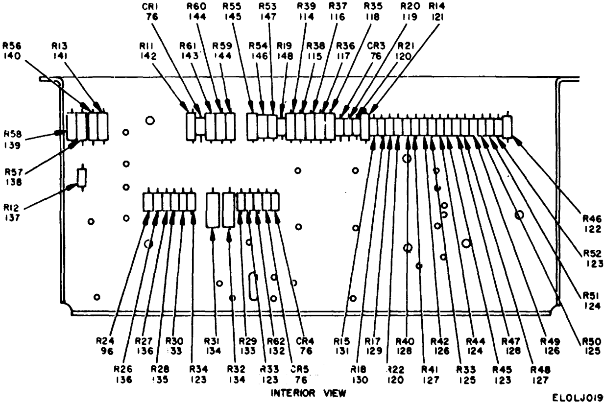
Figure 18. Chassis Assembly (Sheet 3 of 3).
