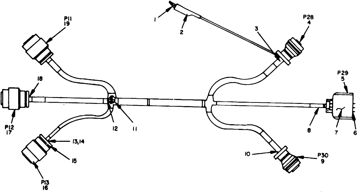
Figure 12. Cable Assembly CX-8792/ASM -125, W11.
