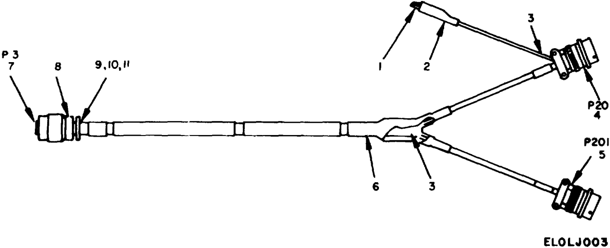
Figure 3. Cable Assembly CX-8786 /ASM-125, W2.
