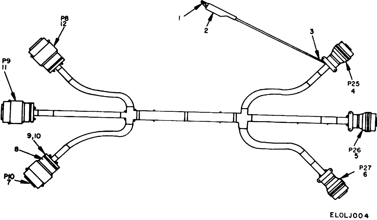
Figure 4. Cable Assembly CX-8791/ASM-125, W3.
