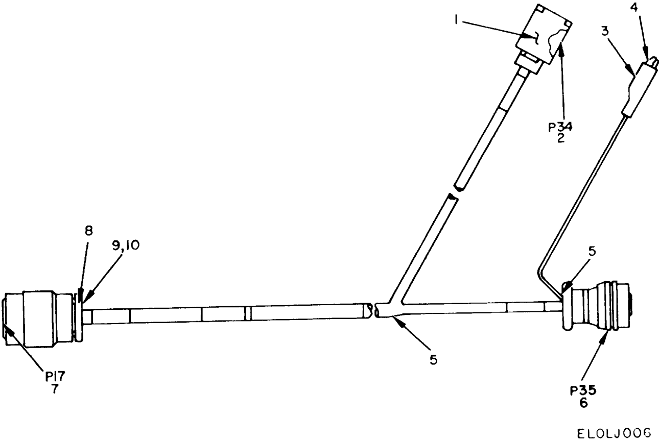
Figure 6. Cable Assembly CX-8795/ASM-125, W5.
