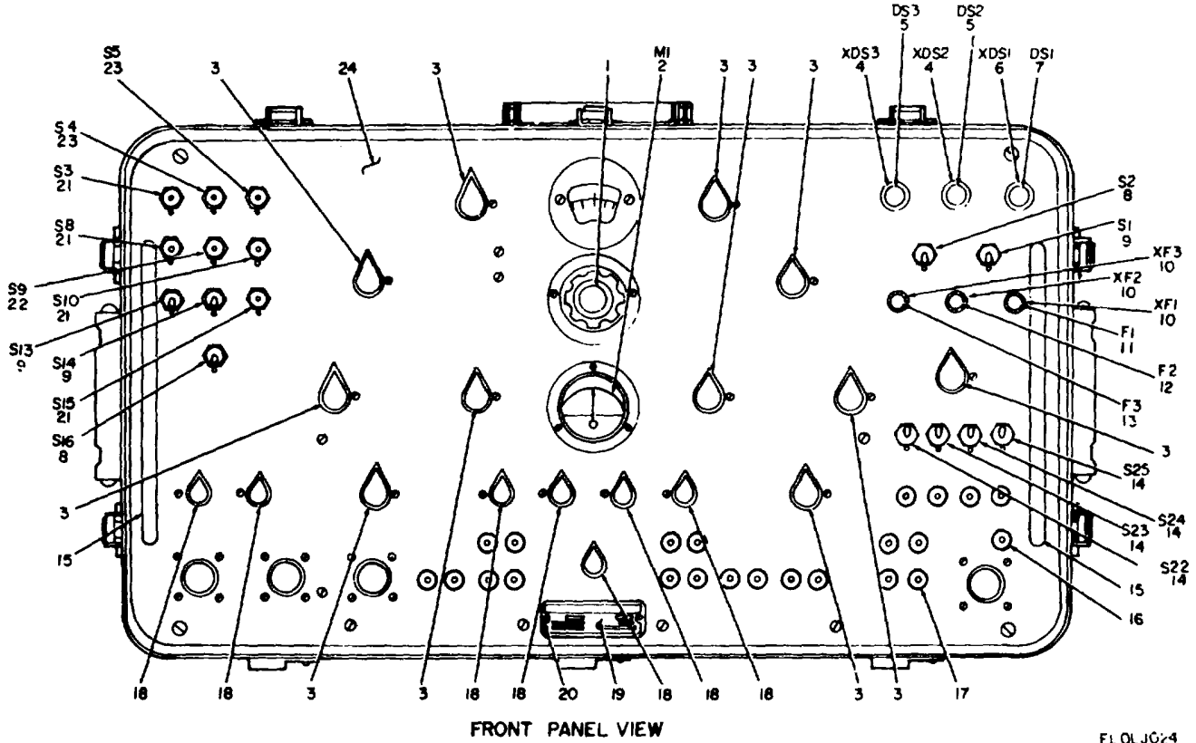
Figure 18. Chassis Assembly (Sheet 1 of 3).
