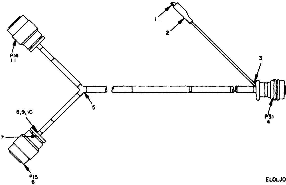
Figure 11. Cable Assembly CX-8793/ASM-125, W10.
