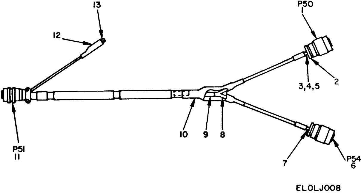
Figure 8. Cable Assembly CX-8782/ASM-125, W7.
