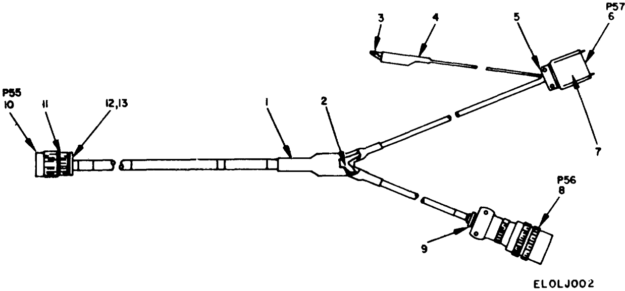
Figure 2. Cable Assembly CX-10100/ASM-125,W1.
